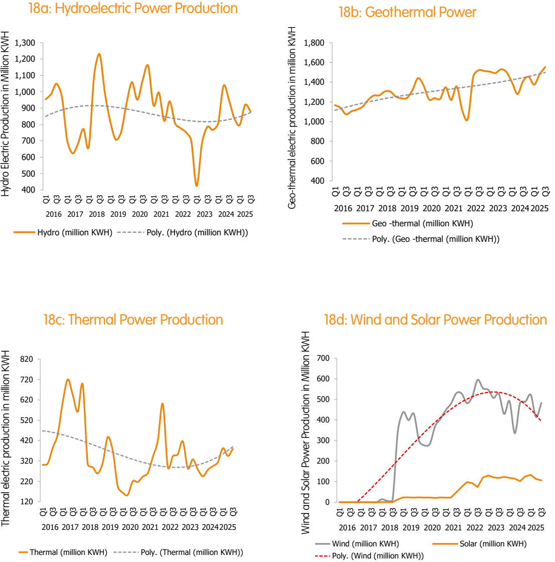
Figure 18 Quarterly Electricity Generation by Source
